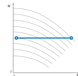
Control for constant pressure
